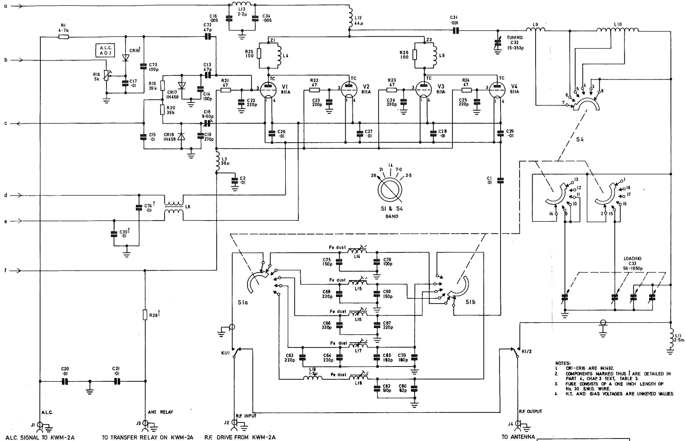
R.F linear amplifier 30L-1 — circuit
